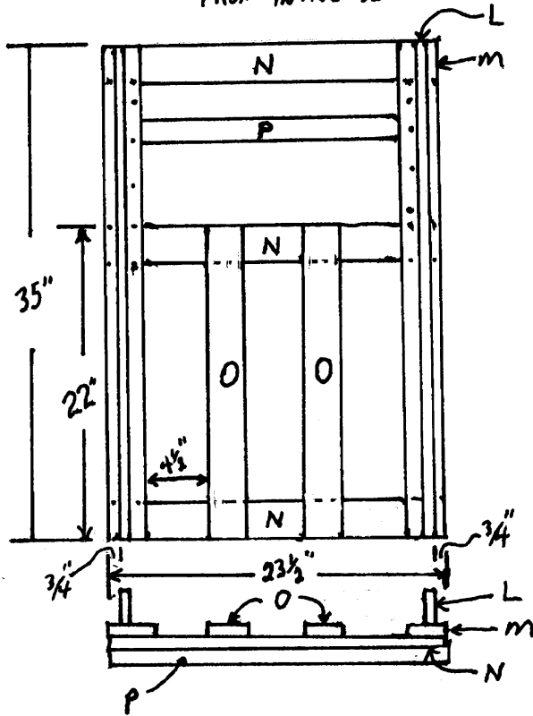
REAR ASSEMBLY FROM INSIDE SLED
